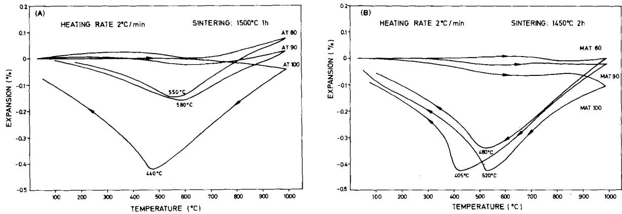
Figure 15 Thermal expansion curves between room temperature and 1000 °C (a) AT-series, sintering: 1500 °C 1 h (b) MAT-series, sintering: 1450 °C 2 h. Heating rate 2 °C min -1 .
